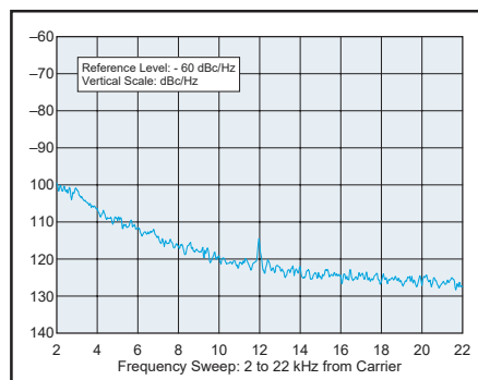
Figure 5—Worst-case VHF/UHF spectral display of the TS-2000 transmitter output during composite-noise testing. Power output is 50 W at 430.02 MHz. The carrier, off the left edge of the plot, is not shown. This plot shows composite transmitted noise 2 to 22 kHz from the carrier.
